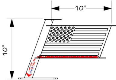
SS-10 STENCIL
